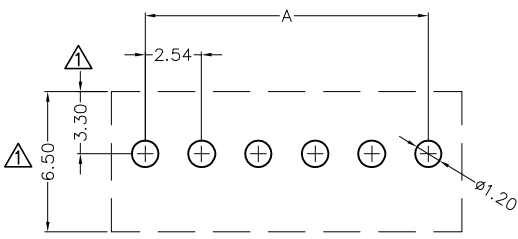
Recommended P.C.Board Layout General Tolerances: ±0.05
